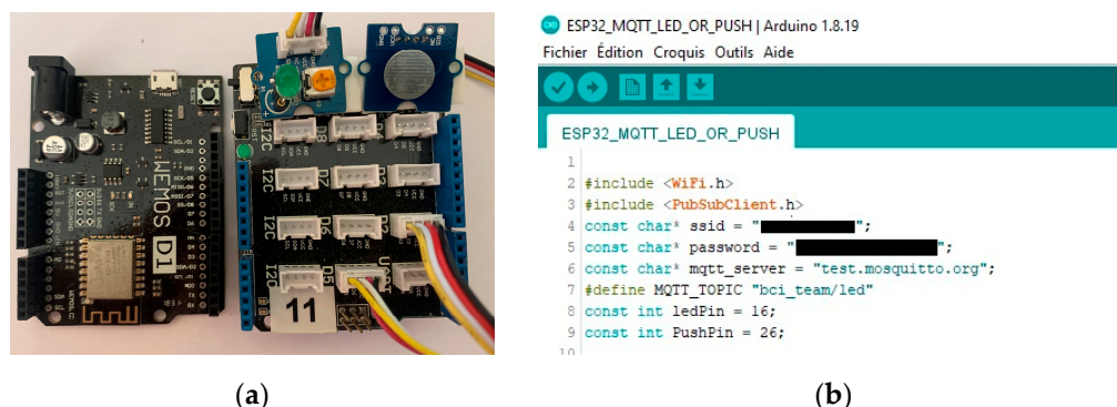
Figure 5. (a) ESP board; (b) MQTT Arduino-based programming.
