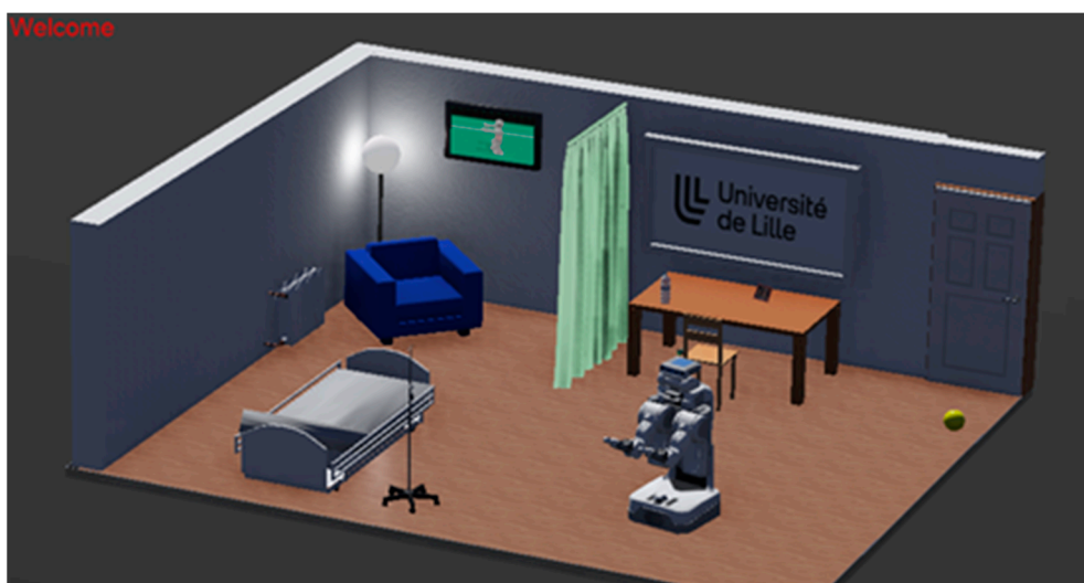
Figure 20. Webots virtual world with interactive objects (lamp, curtain, bed) and PR2 Robot.
