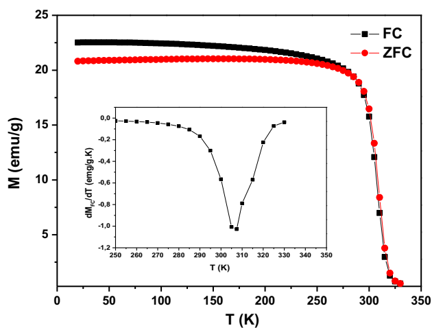
Figure 3. Temperature dependence of magnetization under an applied magnetic field of 0.05T of \text{La}_{0.75}\text{Ho}_{0.05}\text{Sr}_{0.2}\text{MnO}_3 sample. The inset shows the temperature dependence of dM_{FC}/dT .
