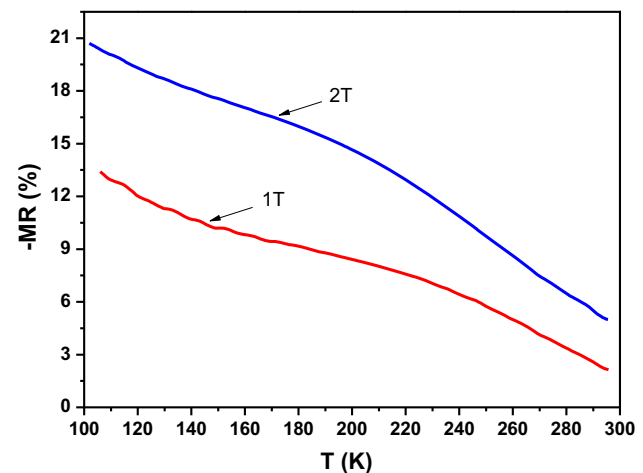
Figure 7. Temperature dependence of magnetoresistance under several values of applied magnetic field for \text{La}_{0.75}\text{Ho}_{0.05}\text{Sr}_{0.2}\text{MnO}_3 sample.
