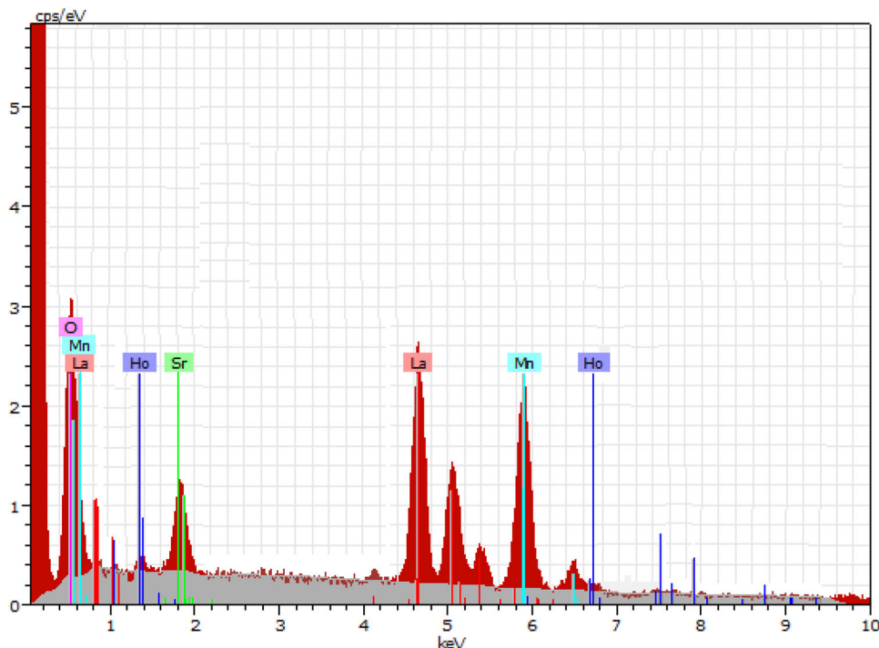
Figure 2. Energy-dispersive X-ray of \text{La}_{0.75}\text{Ho}_{0.05}\text{Sr}_{0.2}\text{MnO}_3 sample.
