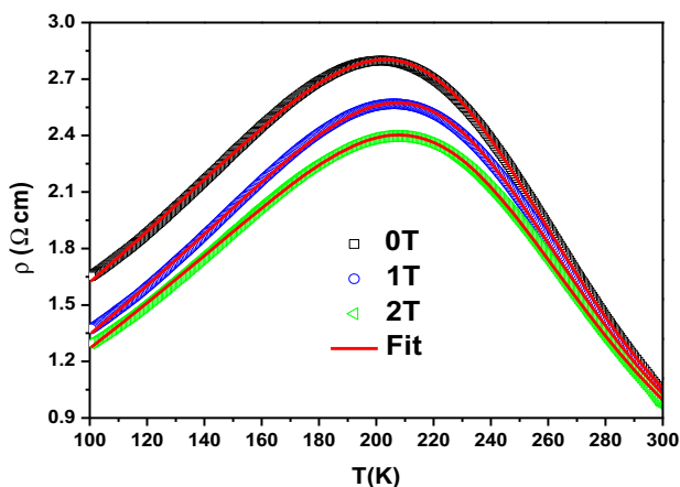
Figure 5. Temperature dependence of electrical resistivity for several values of applied magnetic field for \text{La}_{0.75}\text{Ho}_{0.05}\text{Sr}_{0.2}\text{MnO}_3 sample. The red curves represent the fitting using relation (7).
