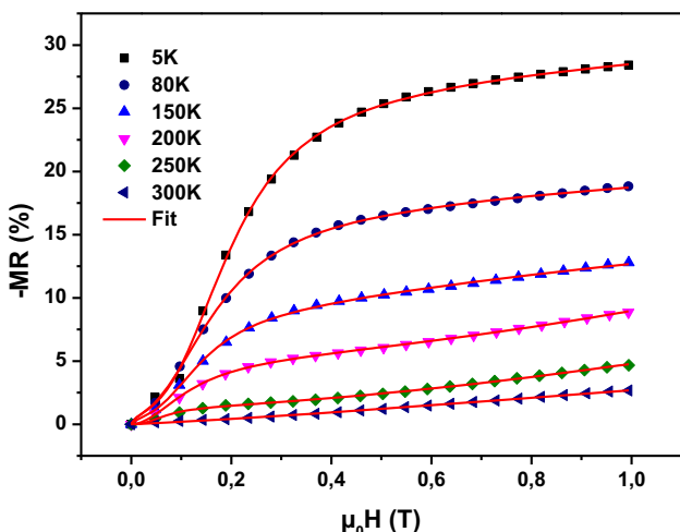
Figure 9. Magnetic field dependence of isothermal magnetoresistance for \text{La}_{0.75}\text{Ho}_{0.05}\text{Sr}_{0.2}\text{MnO}_3 sample. The red curves represent the fitting using relation (9).
