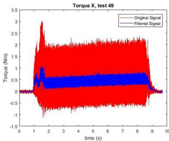
Fig. 4. Measured torque in the x-axis
