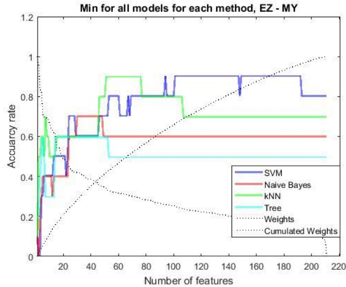
Fig. 6: Worst accuracy result for each algorithm, depending on the number of classified features
