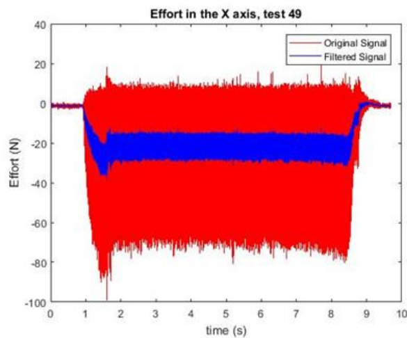
Fig. 3. Measured effort in the x- axis
