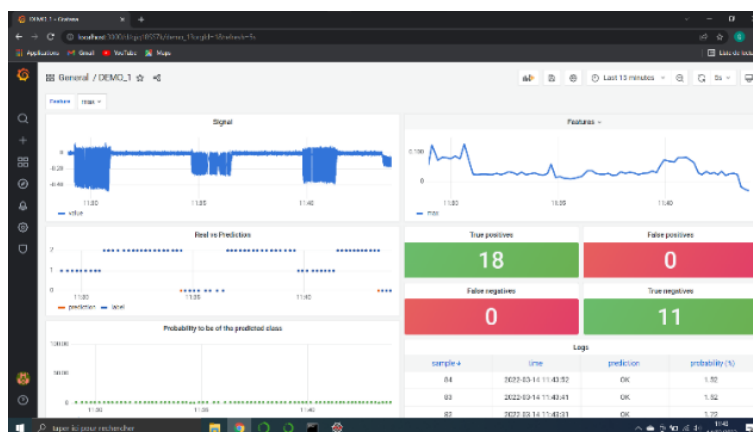
Fig 9: Example of a supervision destined to the model developers
