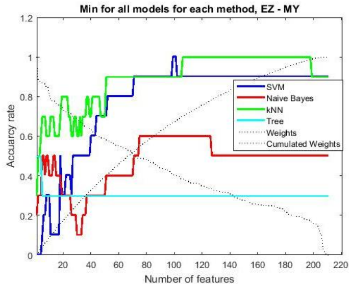
Fig. 5: Worst accuracy result for each algorithm, depending on the number of classified features
