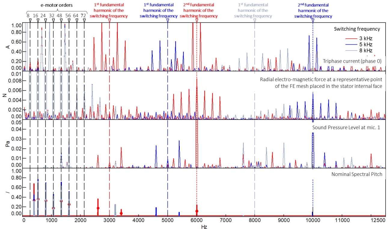
Figure 3: Comparison of results obtained by setting three different switching frequency. Speed is set to 2000 rpm, torque to 50 Nm, while the modulation scheme is the continuous space vector (SVPWM). Axes limits are set to highlight the effect of PWM.
