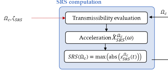
Figure 5: Definition of the SRS computation parameters.
