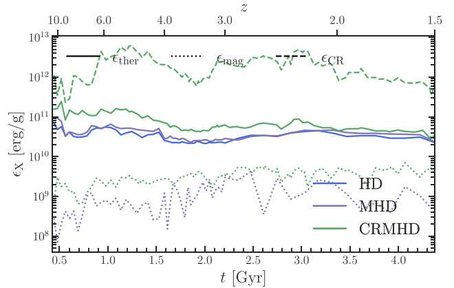
Figure 6. Evolution of specific thermal (solid), magnetic (dotted), and CR (dashed) energies within the galactic region ( 0.2 R_{\text{vir,DM}} ) of NUT. We compare HD (blue line), MHD (purple lines), and CRMHD (green lines) runs. Thermal specific energy shows a decrease of a factor of \sim 3 – 4 between high and low redshift, with the CRMHD specific thermal energy consistently higher than that of the other two runs down to z \sim 2 . From very early on, the CR specific energy clearly dominates ( \sim 1 – 2 dex above thermal specific energy) the energy budget in the CRMHD simulation. Magnetic specific energy plays a secondary role, being well below thermal or CR specific energies at all times and in all runs. Both CRMHD and MHD run exhibit a weak increase in magnetic specific energy with cosmic time.
