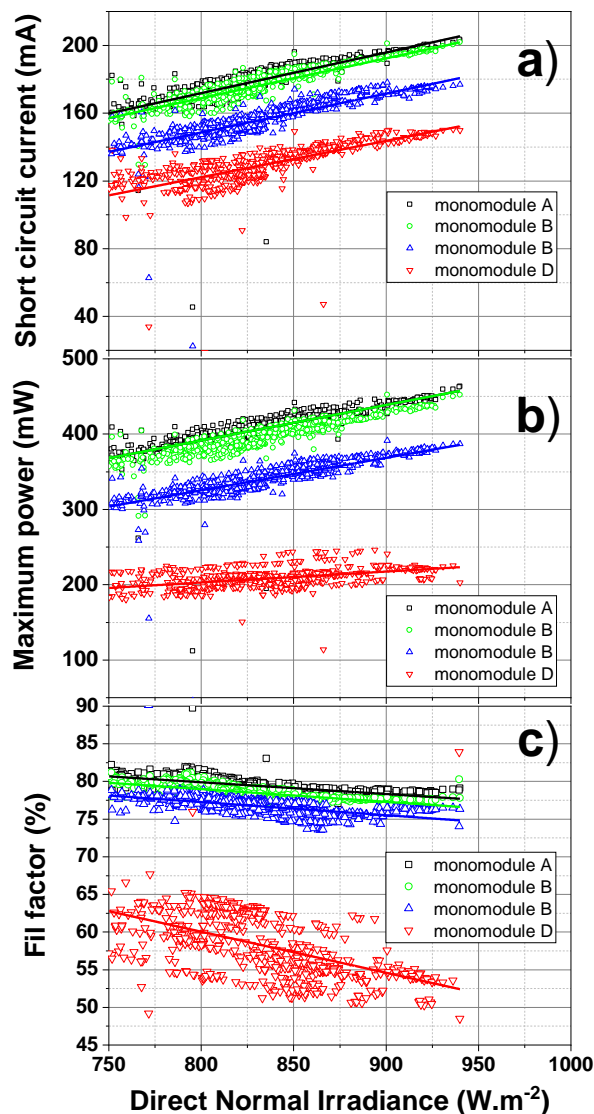
Figure 2: (a) Short-circuit current, (b) Maximum power point and (c) fill factors as a function of DNI of 250× CPV monomodules after data filtering according to ASTM E2527 method described by the IEC 62670-3 standard (mid-August to mid-September 2022).
