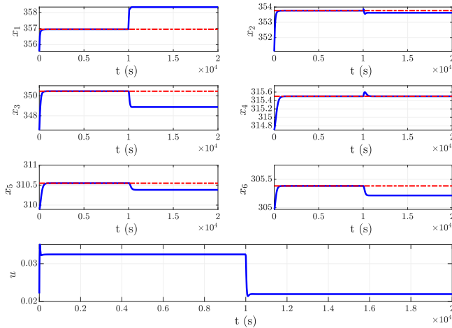
Fig. 3. Evolution of the temperatures of the the heat exchanger cells and the control effort with input and output regulation processes.
