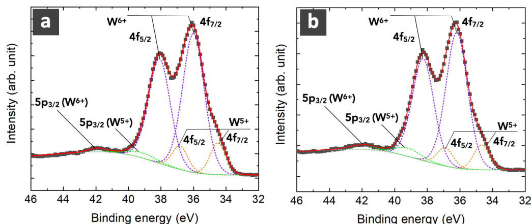
Figure S4. XPS spectra ( W\ 4f band) of two freshly prepared samples (two batches processed with the same solvothermal conditions) with the peak deconvolution giving a stoichiometry WO_{2.93} and WO_{2.94} , respectively (experimental data: black squares; fit: red line; deconvolution: dashed lines).
