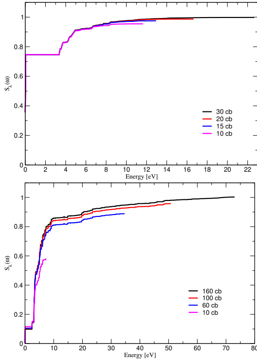
FIG. 9: Cumulative sums S_{\lambda}(\omega) as a function of number of conduction bands (cb) in the BSE hamiltonian for the lowest energy bright exciton in the z direction for (top panel) the optical spectrum (bottom panel) and the XANES spectrum at the L_{2,3} edge. In each case, the zero of the energy axis has been set to the smallest independent-particle transition energy and S_{\lambda}(\omega) has been normalised to its largest value.
