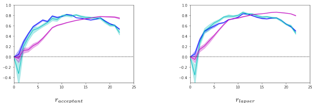
Figure 4: td-BSS of models trained on \mathcal{D}_{train}^{last} and tested on \mathcal{D}_{test}^{last}
