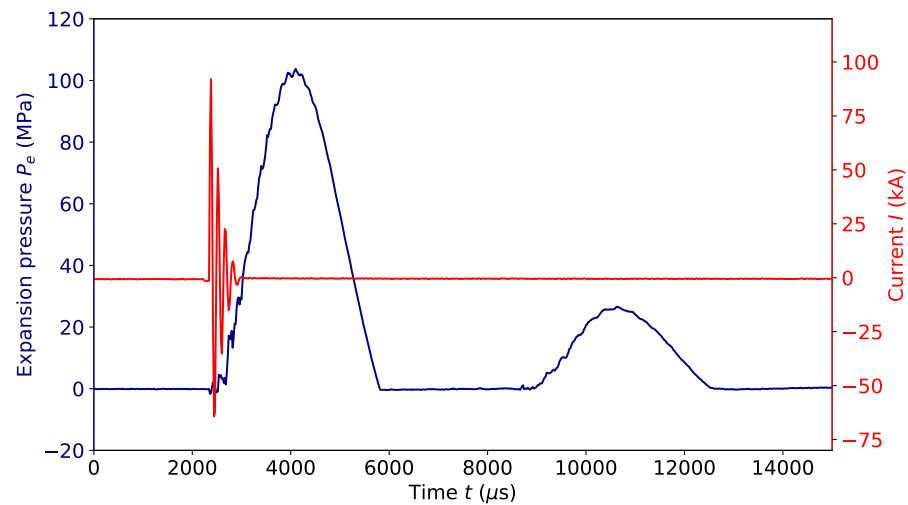
Figure 12. Time evolution of the expansion pressure P_e at the outlet of the crimping probe closed by a rigid ring with the MPS ( E = 8 \text{ kJ} ; e = 2.5 \text{ mm} ).
