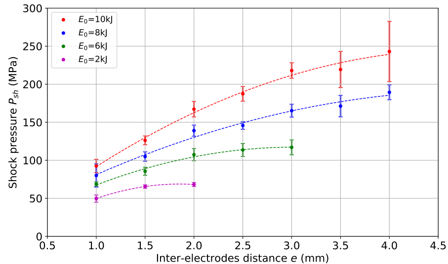
Figure 10. Evolution of the pressure P_{sh} as a function of the inter-electrodes distance e and the discharge energy E_0 .
