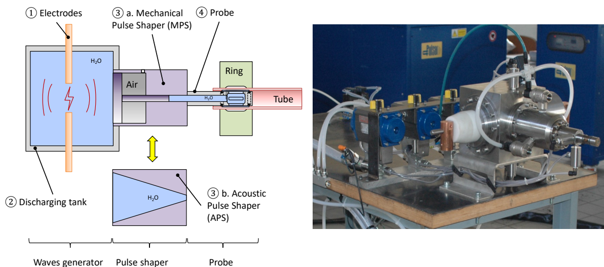
Figure 1. Schematic of electrohydraulic crimping equipment.
