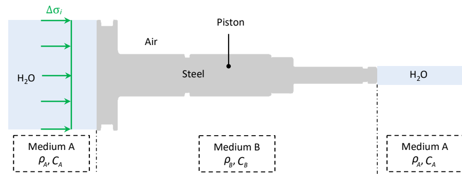
(a) Wave transmission through Mechanical Pulse Shaper
