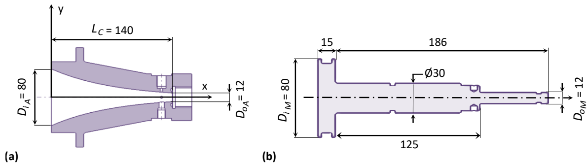
Figure 2. (a) Acoustic and (b) Mechanical Pulse Shapers (units are millimeters).
