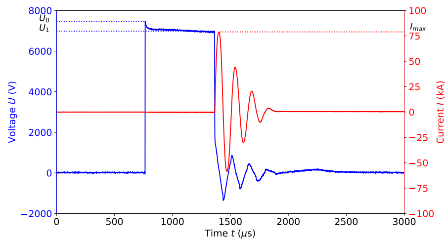
Figure 9. Measure of the discharge current I and the voltage U between the electrodes of the waves generator.
