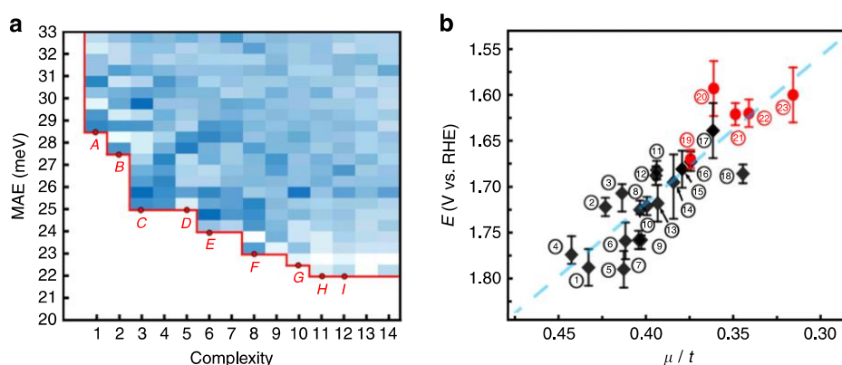
Figure 6 a) Density plot and Pareto front of the mean absolute error as a function of the complexity of 8640 mathematical formulas. B) Onset potentials for the OER reaction as a function of the ratio between the octahedral and tolerance factors ( \mu/t ) (black: previously known perovskites; red dots: discovered perovskites). Reproduced from ref 87 .
