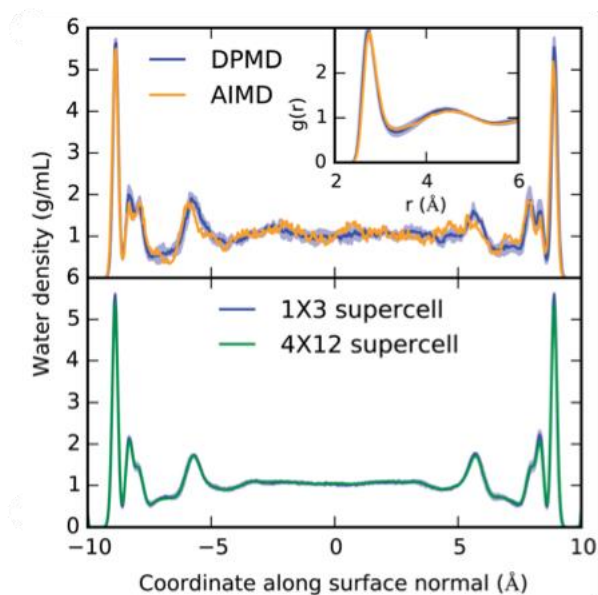
Figure 2 Example of interfacial structure and the effect of long sampling times at the MLP level compared to short sampling at the DFT level. Top: The density profile of water confined between two \text{TiO}_2 surfaces and the oxygen radial distribution functions as obtained from DFT and from an MLP are compared. Statistics were accumulated over 40 ps. Bottom: Equivalent density profile, but this time obtained from an equilibrated 2.5 ns molecular dynamics run. Note the differences for the “second” layer, which depends strongly on the phase-space sampling and only minimally on the chosen unit-cell size. Reproduced from ref 22
