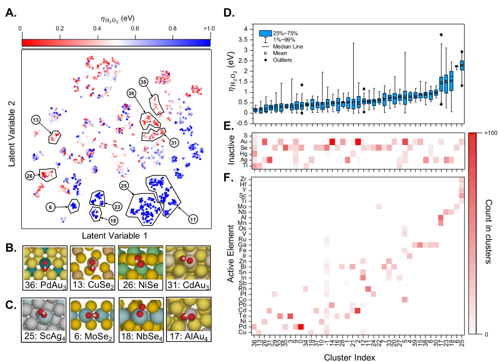
Figure 5. (A) Two-dimensional latent space of surfaces with competitive thermodynamic overpotentials for the production of \text{H}_2\text{O}_2 , \eta_{\text{H}_2\text{O}_2} . Examples of catalytically (B) active and (C) inactive surfaces. (D) Box plot of \eta_{\text{H}_2\text{O}_2} distribution in each cluster and occurrence heatmaps of (E) inactive and (F) active elements in each cluster. Reprinted (adapted) with permission from 57. Copyright 2021 American Chemical Society.
