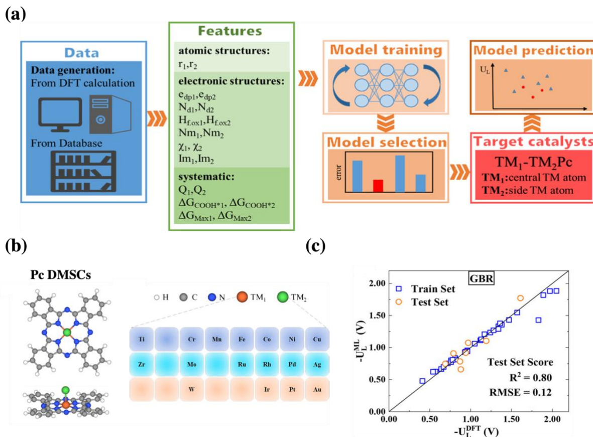
Figure 4 (a) Schematic procedure of the machine-learning-accelerated prediction of catalytic activity of dual metal phthalocyanines, whose structure is illustrated in (b). (c) presents the parity plot and linear regression between the DFT reference data and the best performing gradient boosting regression (GBR) model for the limiting potential U_L for CO_2 electroreduction. Reprinted (adapted) with permission from 48. Copyright 2021 American Chemical Society.
