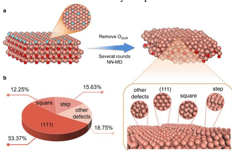
Figure 3 Example of construction of disordered surfaces (here oxide derived Cu) and the statistics of the obtained local active sites. Color code: Brown: Cu, blue : surface O, red: subsurface and bulk O. Reproduced from ref 25 .
