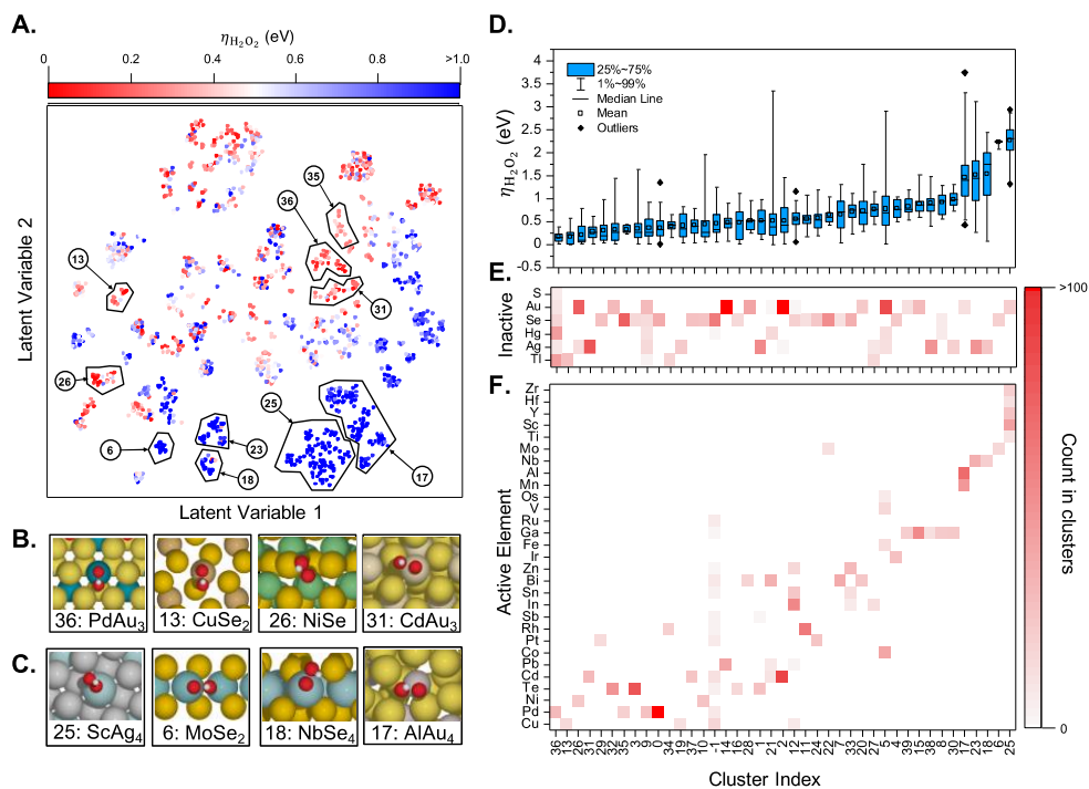
Figure 5. (A) Two-dimensional latent space of surfaces of surfaces with competitive thermodynamic overpotentials for the production of H_2O_2 , \eta_{H_2O_2} . Examples of catalytically (B) active and (C) inactive surfaces. (D) Box plot of \eta_{H_2O_2} distribution in each cluster and occurrence heatmaps of (E) inactive and (F) active elements in each cluster. Reprinted (adapted) with permission from 57. Copyright 2021 American Chemical Society.
