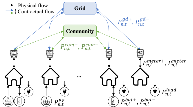
FIGURE 2. Typical energy community architecture.
