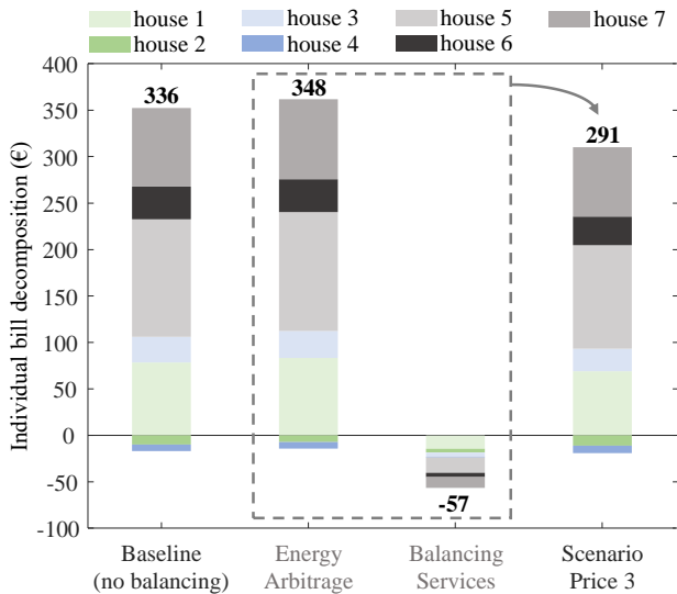
FIGURE 7. Individual bill decomposition for Scenario 3 with equal individual bill savings of 12%.
