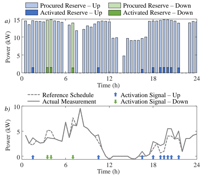
FIGURE 6. a) Balancing capacity and activated energy and b) Reference and measurement curve at the community level for a sample day.
