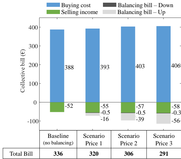
FIGURE 5. Total community bill with positive values mean cost and negative values mean revenue.
