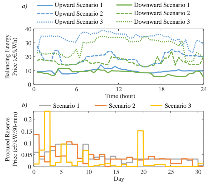
FIGURE 4. a) Balancing energy prices over a sample day, b) Procured reserve prices for all days in the month.
