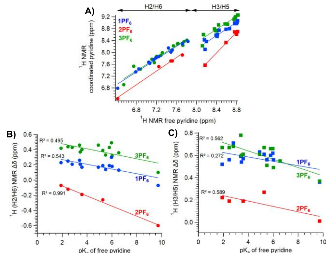
Figure 3. A) Relation between the ^1\text{H} NMR shifts of the H2/H6, H3/H5 protons of coordinated and free pyridines (almost-linear dependence ( R^2 > 0.90 )). Shift of the ^1\text{H} NMR shift between the pyridinic proton in position B) 2/6 or C) 3/5 of the coordinated pyridines vs. the pK a of the free pyridines. For R substituents in ortho or meta position (pyridines k-n ), the most deshielded proton was considered.
