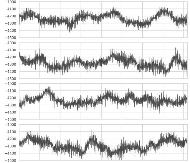
Figure 6. Glitch-free snippets of the seismic data from Mars (U component).
