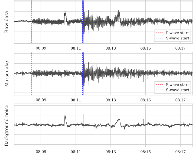
Figure 1. Unsupervised separation of background noise, including thermally induced microtilts (glitches), from a marsquake recorded by the InSight lander’s seismometer on February 3, 2022 (InSight Marsquake Service, 2023). Approximately 30 hours of raw data from the U component, with no recorded marsquakes, were utilized for background noise separation without any explicit prior knowledge of marsquakes or glitches. The horizontal axis represents the UTC time zone.
