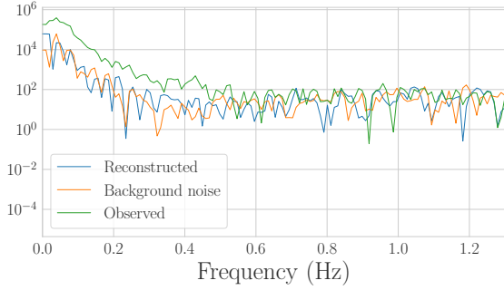
Figure 8. Power spectrum of the observed signal \mathbf{x} , the background noise \mathbf{n} and the reconstructed background noise \mathbf{x} - \mathbf{a}_1^T \tilde{\mathbf{s}}_1 . We see that the reconstructed component statistically agrees with a Mars seismic background noise \mathbf{n} . The algorithm efficiently removed the low-pass component of the signal corresponding to a glitch.
