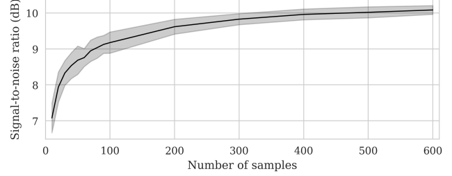
Figure 4. Signal-to-noise ratio of the predicted multifractal random walk data versus number of unsupervised samples. Shaded area indicates the 90% interval of this quantity for ten random source separation instances.
