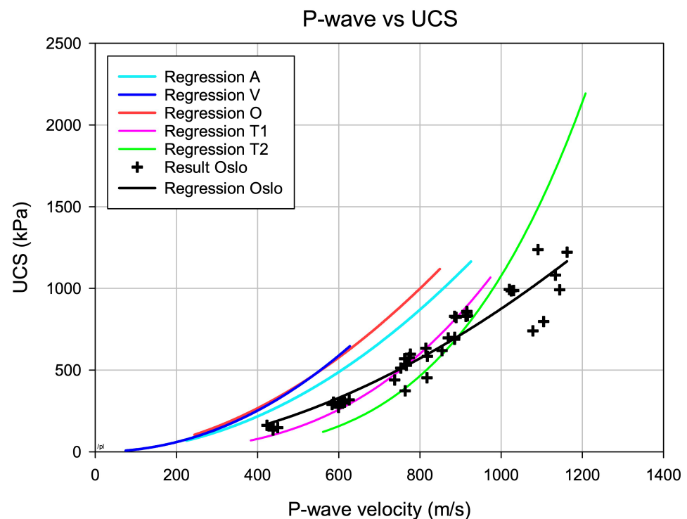
Figure 13. P-wave velocity as a function of the UCS.
