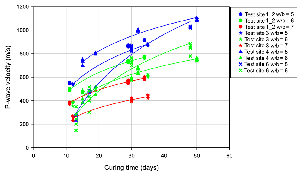
Figure 9. Development of P-wave velocity with curing time for sediment samples stabilized with various water/binder ( w/b ) ratios. Different colour lines show trends in P-wave velocity for stabilised soil samples collected from various test sites.
