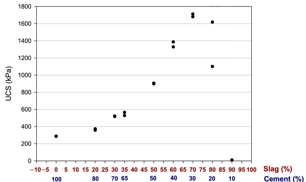
Figure 8. Variation of compressive strength with different proportions between cement and slag. Black dots signify measurements of UCS for soil samples stabilised with different proportions of slag/cement.
