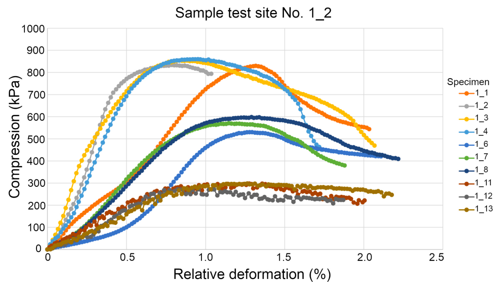
Figure 10. Correlation between compression (kPa) and relative deformation of 10 specimens collected from the sample test site No. 1_2.
