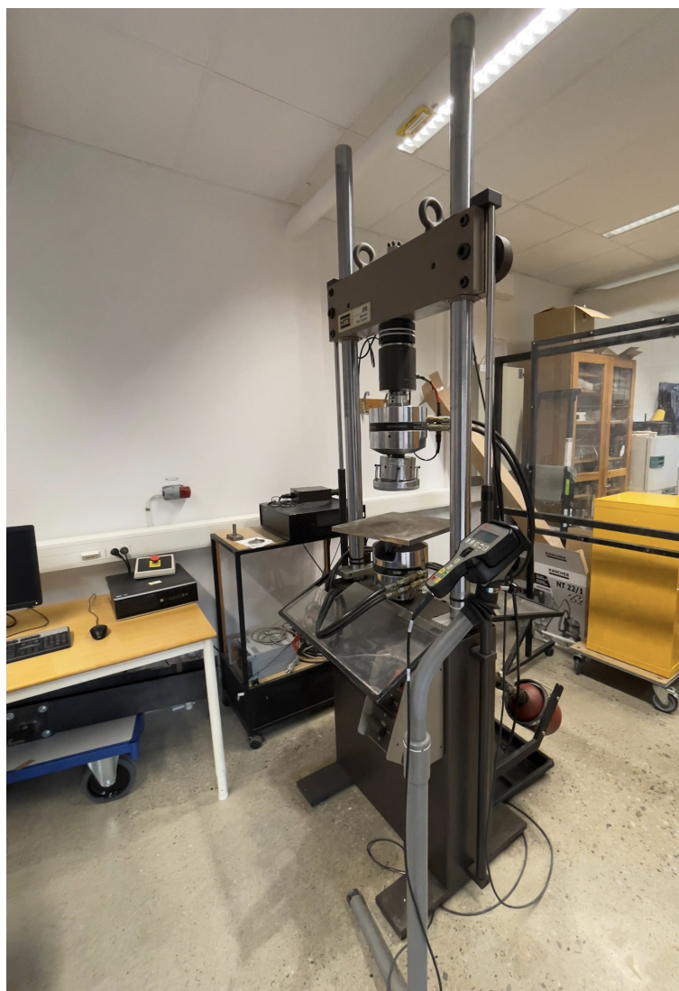
Figure 7. MTS 810 servohydraulic universal testing machine with maximum force capacity of 10 t in compression/tension used for test compressive strength of the specimens. Photo: Per Lindh.
