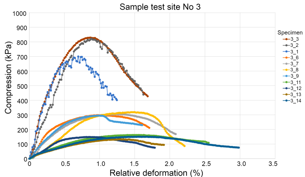
Figure 11. Correlation between the compression (kPa) and relative deformation of 11 specimens from the sample test site No. 3.
