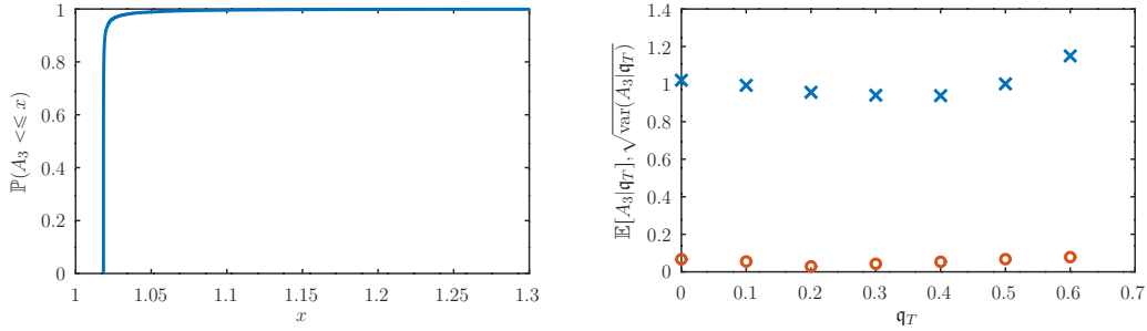
Figure 10: On the left: distribution of A_3 conditioned on \mathbf{q}_T = 0 , on the right: graphs of \mathbb{E}[A_3|\mathbf{q}_T = x] ( \times ) and \text{var}(A_3|\mathbf{q}_T = x)^{1/2} ( o )
