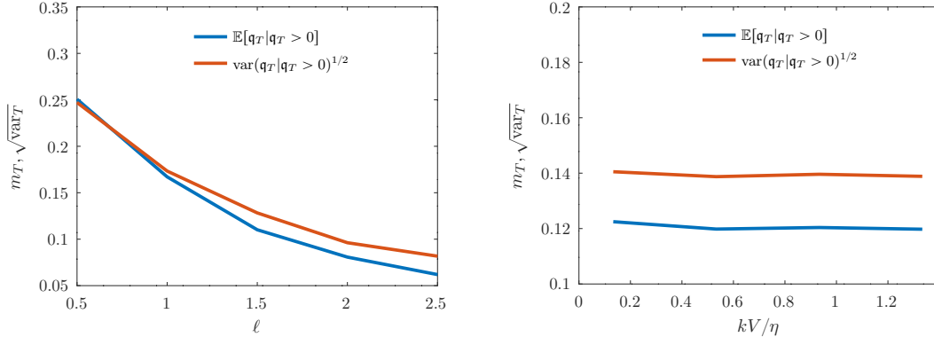
Figure 5: Graph of m_T = \mathbb{E}[\mathbf{q}_T | \mathbf{q}_T > 0] and \sqrt{\text{var}} = \text{var}(\mathbf{q}_T | \mathbf{q}_T > 0)^{1/2} as a function of \ell
