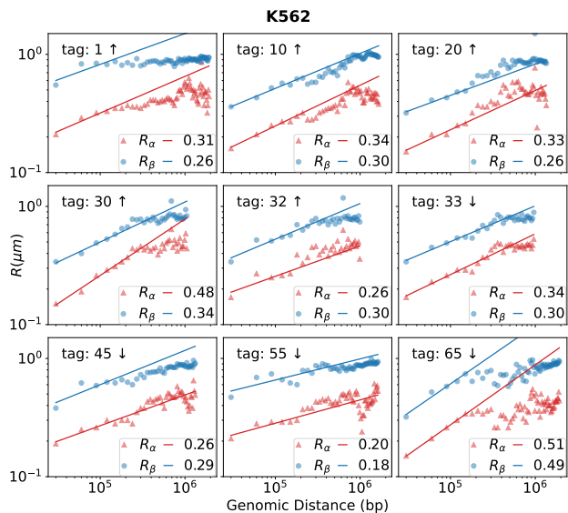
FIG. A.1. Scaling of the characteristic radii of the two phases R_\alpha and R_\beta for a few selected tags in the leukemia cell line K562. The notation is the same as of Fig. 3 with “tag: 10 ↑” means that R_\alpha and R_\beta are calculated for i = 10 and j = 11, 12 \dots N . The solid lines are power-law fits over the the first five points ( s \leq 150 kb).
