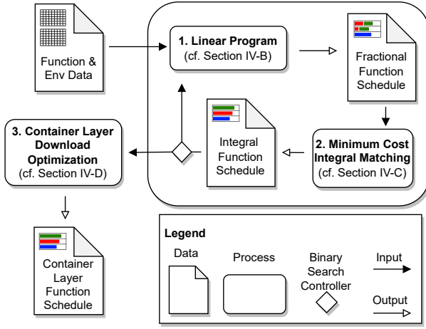
Figure 2: FOA's Algorithm step by step.
