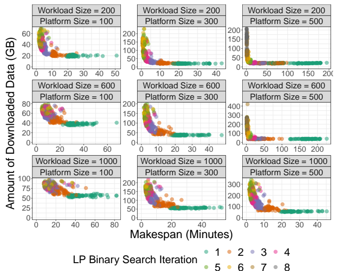
Figure 4: FOA 's linear program trade-off between makespan (x-axis) and amount of downloaded data (y-axis). The color of the points represents the iteration-id of the linear program binary search. Each one is one solution of the linear program.
