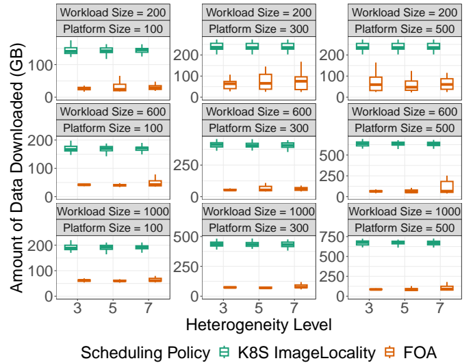
Figure 6: Comparison of K8S ImageLocality and FOA in terms of the amount of downloaded data (y-axis) against the heterogeneity level (x-axis).
