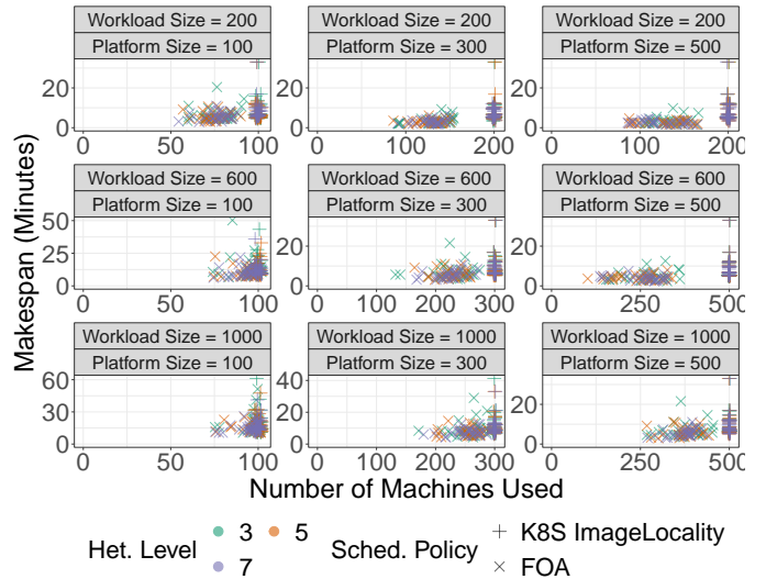
Figure 8: The makespan (y-axis) against the number of machines used (x-axis). Facets combine workload and platform sizes. Shapes represent the scheduling policies, and colors represent the heterogeneity level.
