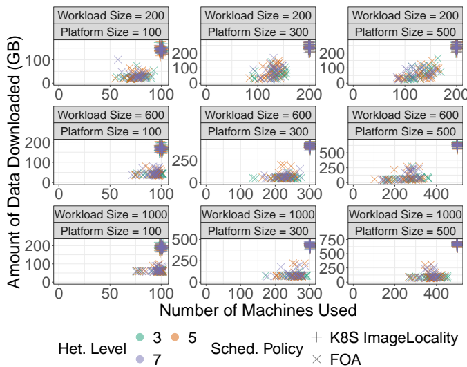
Figure 9: The amount of data downloaded (y-axis) against the number of machines used (x-axis). Facets combine workload and platform sizes. Shapes represent the scheduling policies, and colors represent the heterogeneity level.
