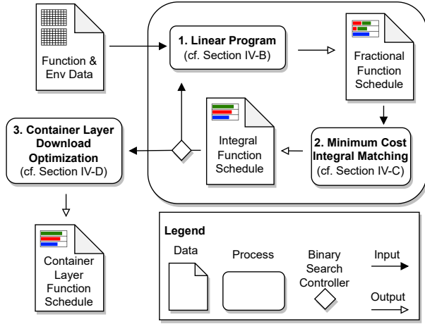
Figure 2: FOA's Algorithm step by step.
