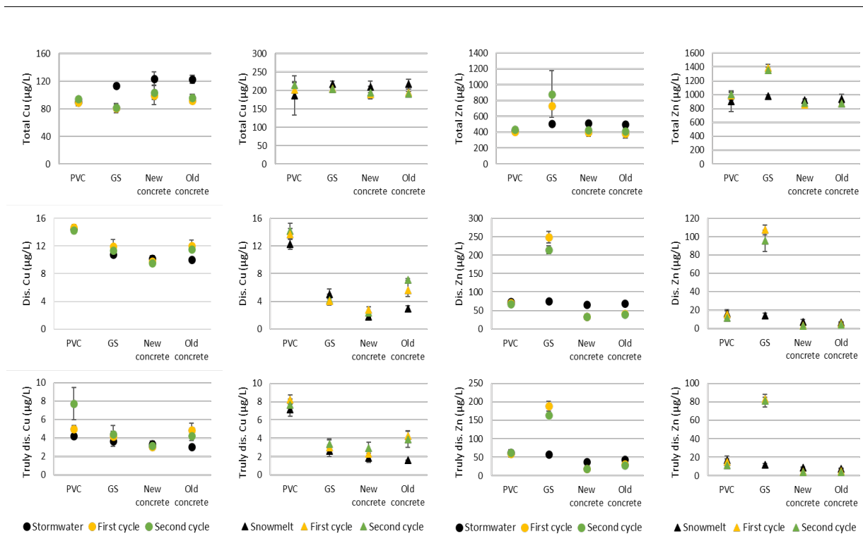
Fig. 1 Changes in total, dissolved and truly dissolved Cu and Zn concentration in stormwater and snowmelt after exposure to pipe materials (black color markers show initial values in stormwater and snowmelt)
