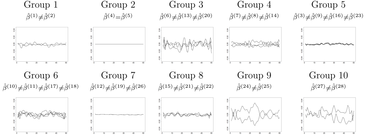
Figure 12: \text{GFUL}_{\text{Euclidean}} estimated coefficients
