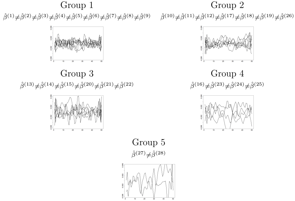
Figure 13: \text{GFUL}_{\text{Circle}} estimated coefficients
