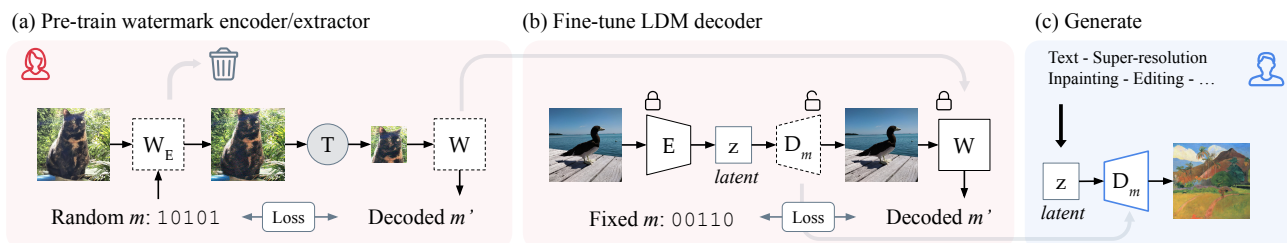
Figure 2. Steps of the method. (a) We pre-train a watermark encoder \mathcal{W}_E and extractor \mathcal{W} , to extract binary messages. (b) We fine-tune the decoder \mathcal{D} of the LDM’s auto-encoder with a fixed signature m such that all the generated images (c) lead to m through \mathcal{W} .
