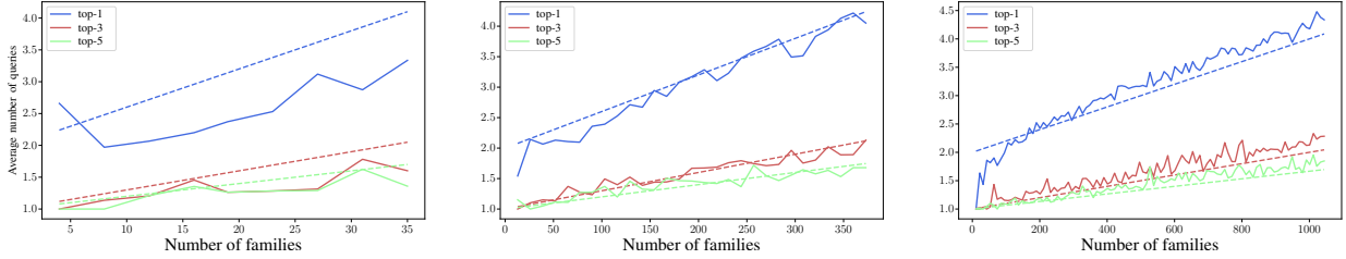
Fig. 4: Average number of queries as a function of the number of families n_{\mathcal{F}} for (I, \mathcal{F}, \mathcal{A} = \mathcal{B}, k) with the expectation score (7) and when the black-box returns top- k classes with k = 1 (blue), k = 3 (red) or k = 5 (green). The dotted lines represent the linear regressions (13). Family considered from left to right: \mathcal{F}(m) (3), \mathcal{F}(m, \Psi) (4), and \mathcal{F}(m, \{\theta\}) (5).
