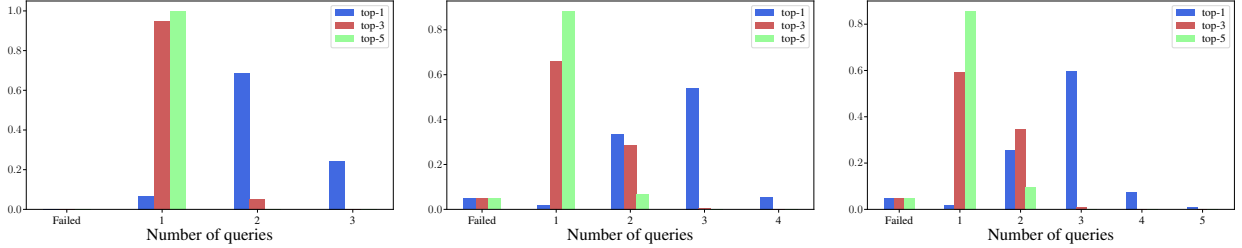
Fig. 3: Probability distribution of the number of queries for (I, \mathcal{F}, \mathcal{A} = \mathcal{B}, k) when the black box returns top- k classes with k = 1 (blue), k = 3 (red) or k = 5 (green). Family considered from left to right: \mathcal{F}(m) (3), \mathcal{F}(m, \Psi) (4), and \mathcal{F}(m, \theta) (5).
