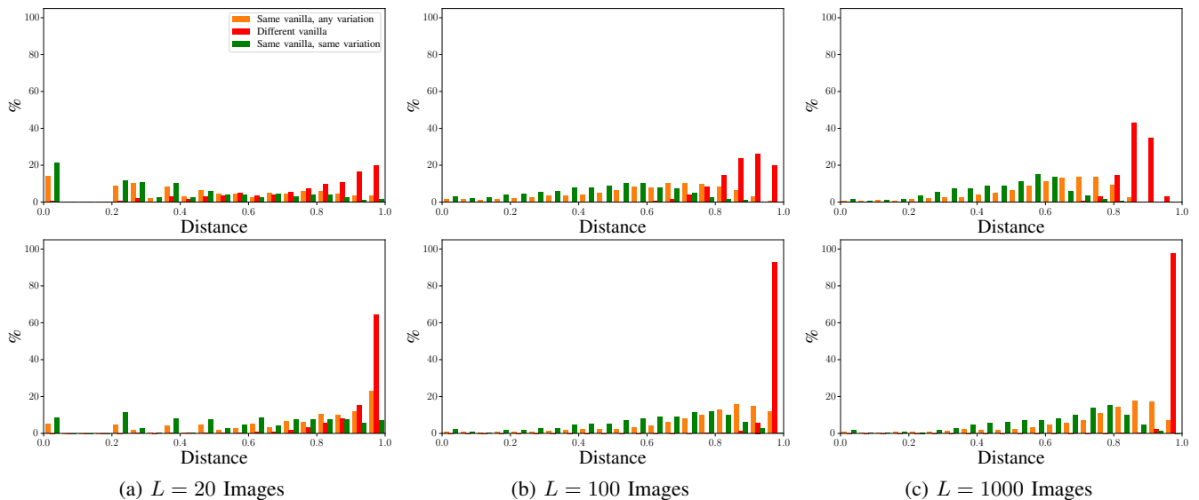
Fig. 5: Histogram of the distance D_L(m_1, m_2) when (m_1, m_2) \in \mathcal{F}^2(m) (orange), (m_1, m_2) \in \mathcal{F}^2(m, \Psi) (green), or m_1 and m_2 are variants of different vanilla models (red). Inputs randomly sampled in \mathcal{X} ( top ) or in \mathcal{X}' -Entropy Sect. IV-B2- ( bottom ).
