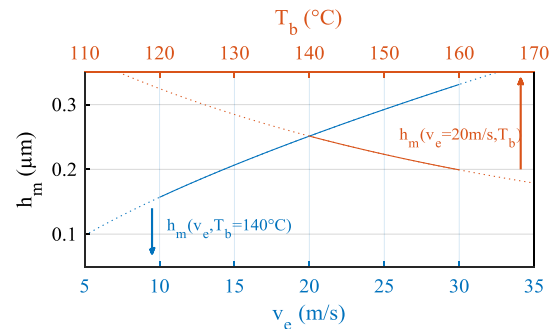
Figure 16: Variation of the film thickness as analytical functions of the temperature and entrainment speed for given operating conditions
