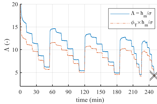
Figure 17: Reduced film thickness evolution during the test
