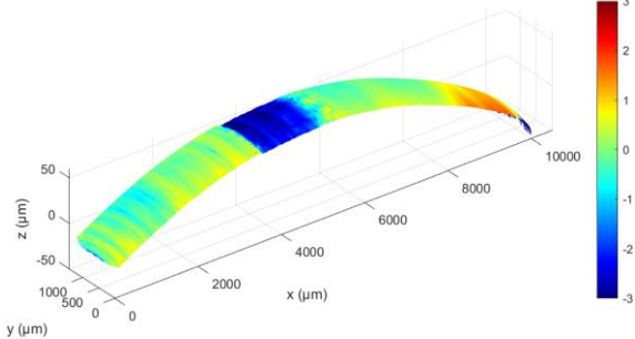
Figure 12: Measured surface, deviation from a crowned disk, slow surface
