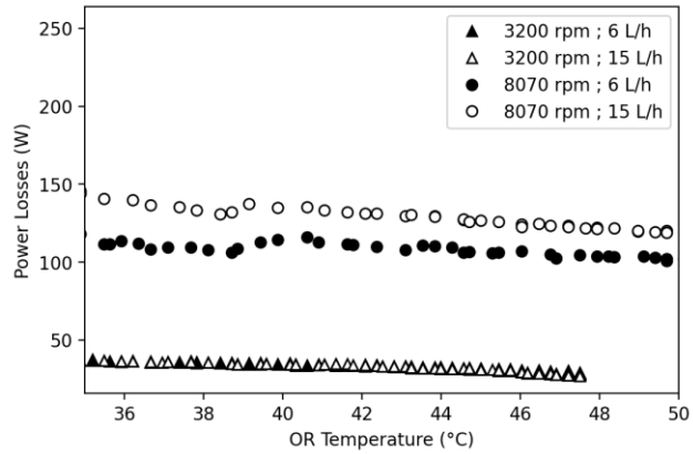
Figure 10 Power losses versus the outer ring temperature of the REB #2 for two speeds (3200 and 8070 rpm) and for two oil flow rates (6 and 15 L/h), with oil at 25°C
