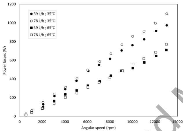
Figure 3 Power losses versus the rotational speed, results from [21], with oil flow rate and lubricant initial temperature
