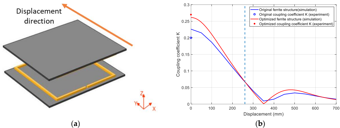
Figure 21. Comparison of the coupling coefficient K between the original ferrite structure and optimized ferrite structure: (a) displacement along the y -axis; (b) comparison of the coupling coefficient K between the original ferrite structure and optimized ferrite structure along the y -axis.
