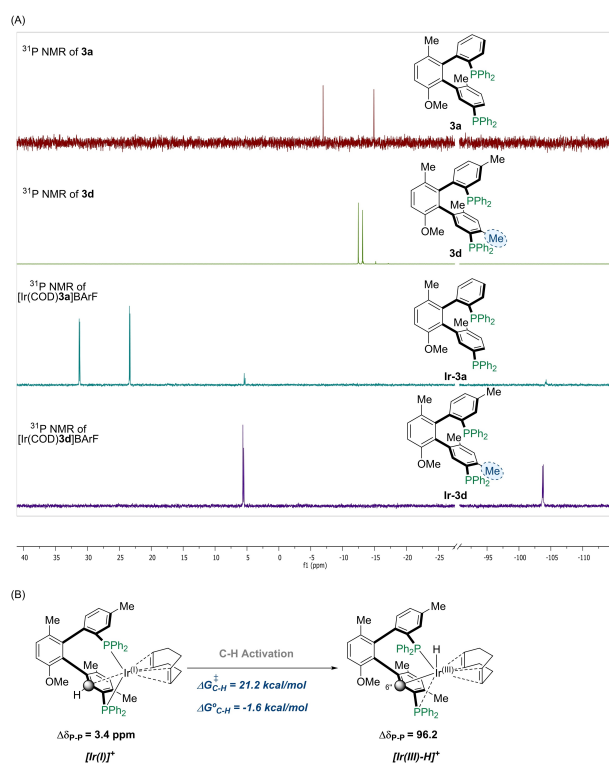
Scheme 6. (A) 31 P NMR of 3a , 3d , [Ir(COD) 3a ]BARF and [Ir(COD) 3d ]BARF; (B) Iridium(I) C–H activation of 3d .
