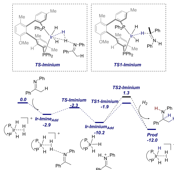
Scheme 8. Free energy profile of outer-sphere imine hydrogenation mechanism (A) for both enantiomers. Energies in kcal/mol.
