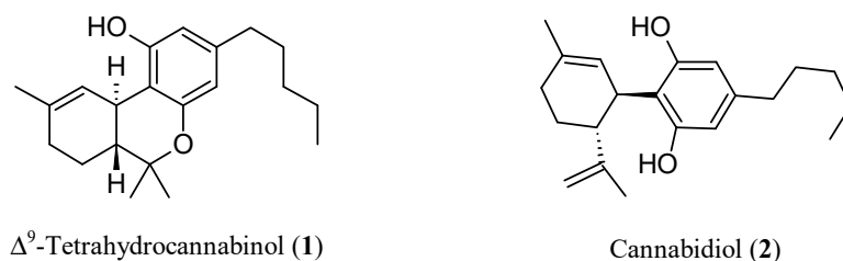
Figure 1. Chemical structures of \Delta^9 -tetrahydrocannabinol (THC, 1) and cannabidiol (CBD, 2).
