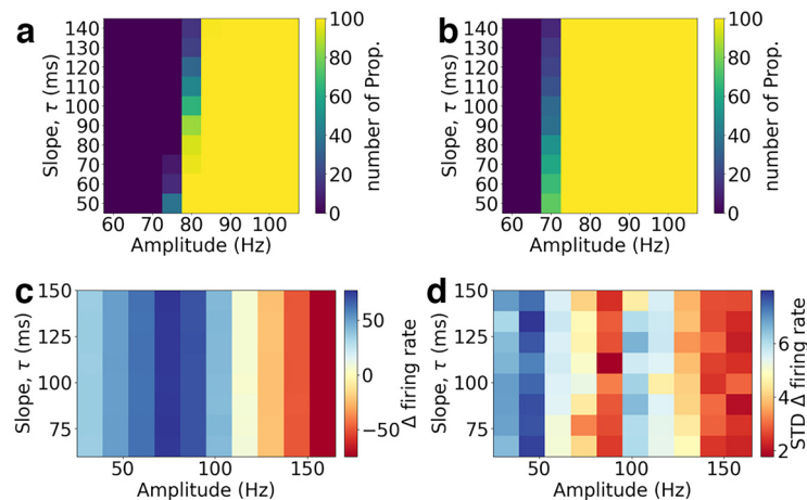
Figure 4. Grid search on the amplitude and slope of the incoming perturbation for each network. a, b , The percentage of realizations that propagate (Prop.), respectively, for AdEx ( a ) and CAdEx ( b ) networks. c, d , For HH networks, the means and SDs (over realizations) of the difference in firing rates between excitatory ( c ) and Poisson ( d ) populations ( \Delta firing rate = \nu_e - \nu_{\text{Pois}} ), averaged over the length of the plateau.
