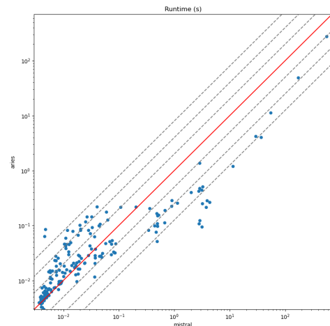
Figure 2. Openshop: Runtime comparison between ARIES and MISTRAL. Dashed lines materialize powers of two runtime differences.
