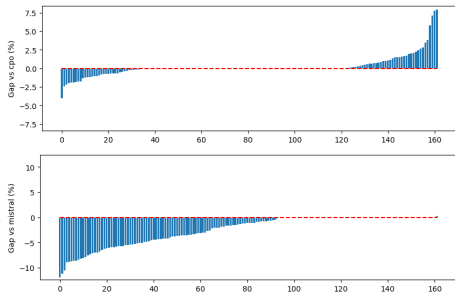
Figure 4. Solution quality variation on jobshop instances. The gap is computed as \frac{(m_1 - m_2) \times 100}{\min(m_1, m_2)} where m_1 is the makespan of the solution found by ARIES and m_2 is the makespan of the solution found by CPOPTIMIZER (resp. MISTRAL). A negative value indicates that ARIES returned a strictly better solution.
