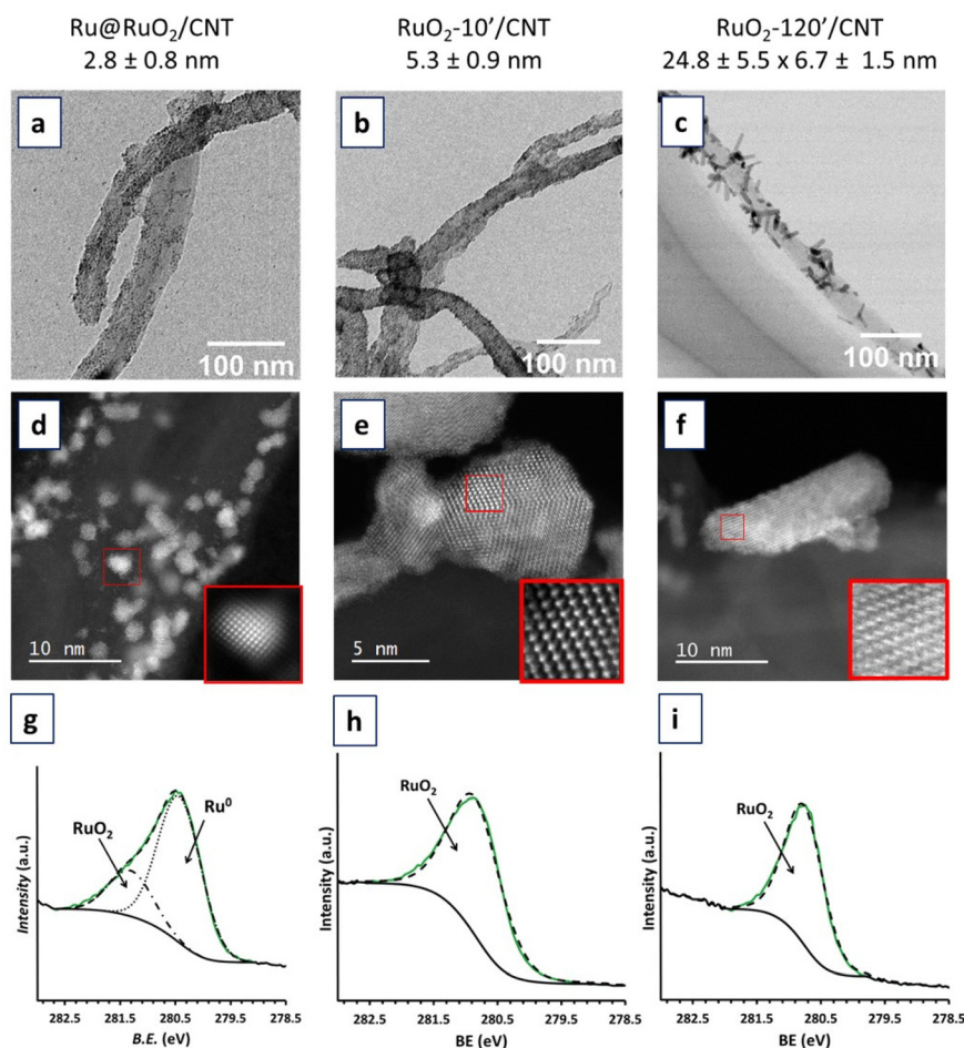
Fig. 2 TEM images, HRTEM images and XPS spectra of \text{Ru@RuO}_2/\text{CNT} (a, d and g), \text{RuO}_2\text{-}10'/\text{CNT} (b, e and h) and \text{RuO}_2\text{-}120'/\text{CNT} (c, f and i) nanostructures. In the XPS spectra, the \text{RuO}_2 component is shown by a dotted-dashed black line, the \text{Ru}(0) component by a dotted black line, the envelope by a dashed black, the experimental data by a solid green line and the background signal by a solid black line.
