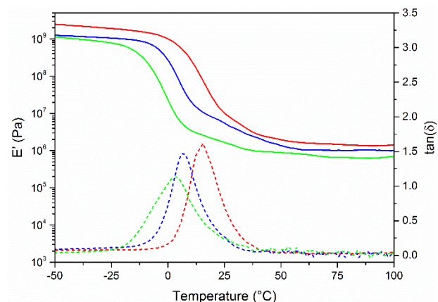
Figure 4. Storage modulus (plain lines) and tan( \delta ) (dashed lines) of FPA-8 (red), FPA-17 (blue) and FPA-25 (green).
