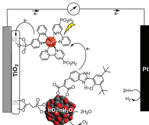
Figure 13. Schematic drawing of a photoelectrochemical OER device based on \text{TiO}_2 photoanodes codoped with phosphonate-derived [\text{Ru}(\text{bpy})_3]^{2+} and \text{IrO}_2 NPs functionalized with a PSII tyrosine-histidine mediator mimic. Adapted with permission. [55] Copyright 2012, PNAS.
