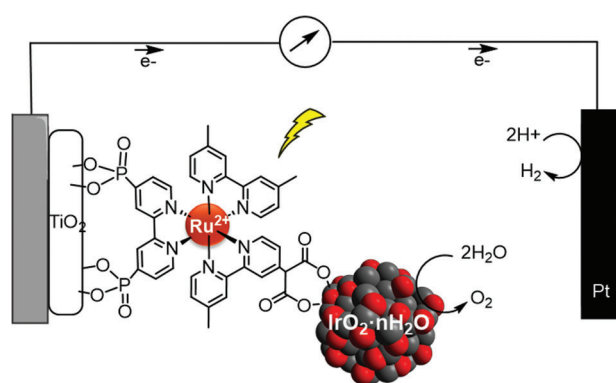
Figure 12. Schematic drawing of a photoelectrochemical OER device based on a \text{TiO}_2 photoanode doped with Ru- \text{IrO}_2 dyads and a Pt cathode. Adapted with permission. [141] Copyright 2009, American Chemical Society.
