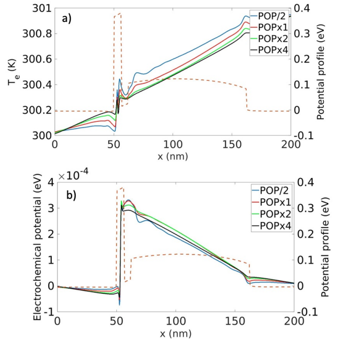
FIG. 9. (Color online) Electron temperature a) and electrochemical potential b) along the device for four different coupling strengths with polar optical phonons: divided by 2 (blue), standard (red), multiplied by 2 (green), and multiplied by 4 (black). The dashed line represents the potential profile. T_{Emit}=300 K, T_{Coll}=301 K and V=0 V.
