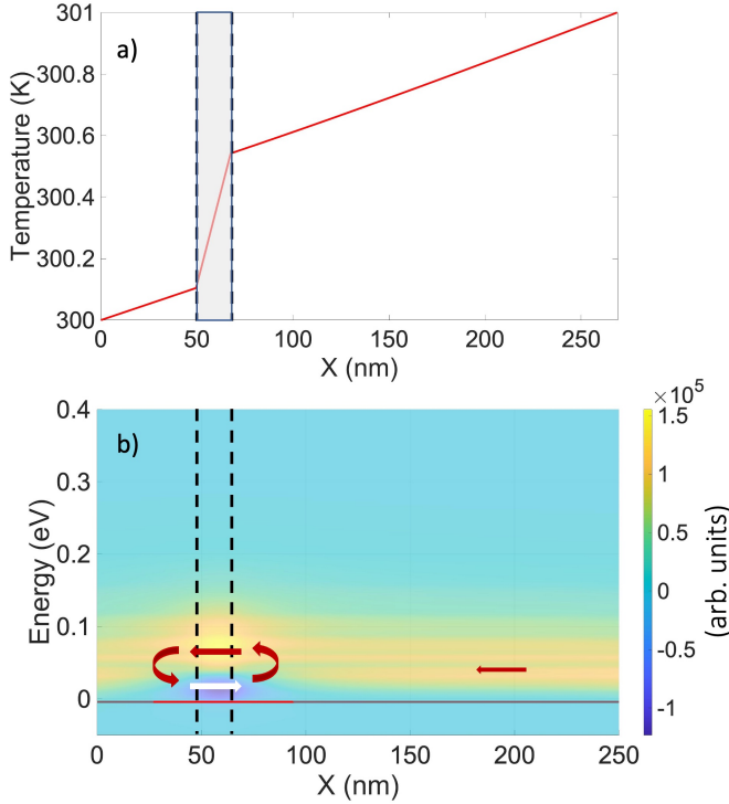
FIG. 12. (Color online) a) Lattice temperature gradient along a GaAs device of the same length as the one of Figure 1, when considering a thermal conductivity of 4 \text{ W.m}^{-1}.\text{K}^{-1} inside the shaded central region. As previously a thermal conductivity of 46 \text{ W.m}^{-1}.\text{K}^{-1} is assumed elsewhere and 1 K is applied between the emitter ( T_{Emit}=300 \text{ K} ) and collector ( T_{Coll}=301 \text{ K} ) reservoirs; b) Corresponding electron current spectrum. The horizontal solid red line represents the energy potential profile, while red and white arrows indicate the electron flow and reflection at the borders where the thermal conductivity varies. The smaller red arrow in the right region represents the total electron flow, going from right to left. No potential bias is applied ( V=0 \text{ V} ).
