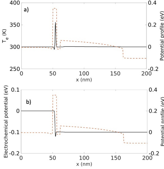
FIG. 6. (Color online) a) Non-equilibrium electron temperature along the device and b) corresponding electrochemical potential when applying a potential bias ( V=0.1 V) and no temperature gradient ( T_{Emit}=T_{Coll}=300 K).
