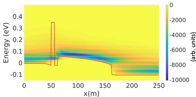
FIG. 4. (Color online) Electron current spectrum for the same previous structure on which a potential bias of V=0.1 V is applied between the emitter and collector reservoirs. No temperature gradient is considered ( T_{Emit}=T_{Coll}=300 K). The solid red line represents the energy potential profile. In this case, the electron goes in the same direction (i.e. from left to right) at all the energies.
