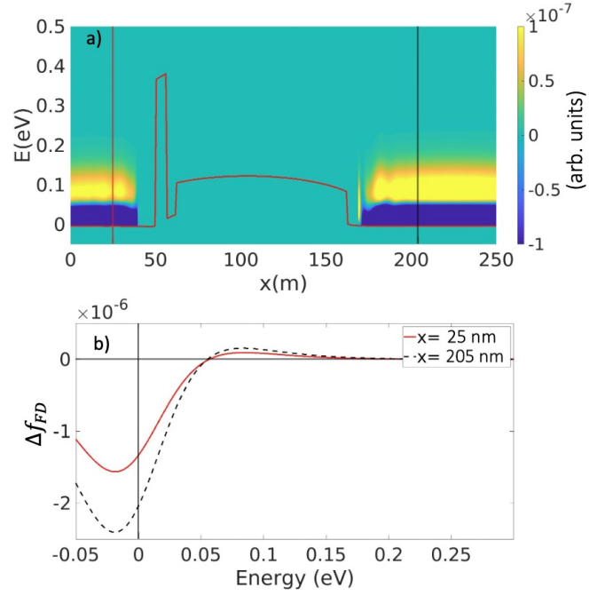
FIG. 7. (Color online) a) Difference between two consecutive plans of the Fermi-Dirac distributions calculated with the electron temperature and chemical potential shown on Fig. 5-a) and -b) respectively; b) Vertical cuts of Fig. 7-a) at x=25 nm (red solid line) and x=205 nm (dashed line). The vertical black solid line defines the Fermi-levels of the emitter and collector (equal since there is no applied bias).
