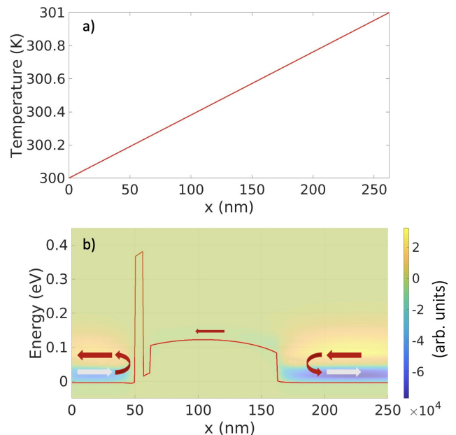
FIG. 2. (Color online) a) Lattice temperature gradient along the device shown in Figure 1. 1 K is applied between the emitter ( T_{Emit}=300 \text{ K} ) and collector ( T_{Coll}=301 \text{ K} ) reservoirs; b) Corresponding electron current spectrum. The solid red line represents the energy potential profile, while red and white arrows indicate the electron flow and reflection on the potential barrier. The smaller red arrow in the central region represents the total electron flow, going from right to left. No potential bias is applied ( V=0 \text{ V} ).
