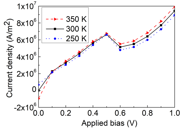
FIG. 10. (Color online) J(V) for three different temperature profiles: i) with a positive 50 K gradient, i.e. T_{Emit}=300 K, T_{Coll}=350 K (triangles); ii) without gradient, where the lattice temperature equals 300 K in all the device (squares); and iii) with a negative 50 K gradient, i.e. T_{Emit}=300 K, T_{Coll}=250 K (circles). We consider the structure of Fig.1 with an aluminum concentration in the collector barrier y=0.2 , corresponding to a barrier height of 160 meV. This higher barrier allows to emphasize the impact of the revolving effect on current characteristics.
