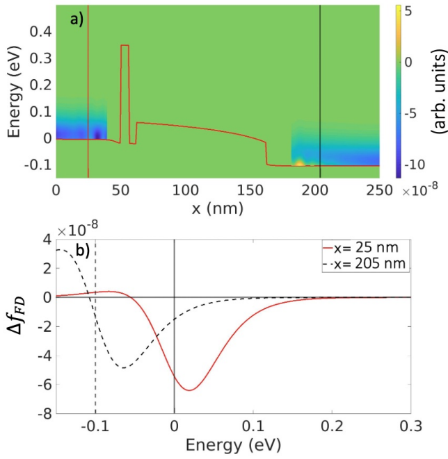
FIG. 8. (Color online) a) Difference between two consecutive plans of the Fermi-Dirac distributions calculated with the electron temperature and chemical potential shown on Fig. 6-a) and-b) respectively; b) Vertical cuts of Fig. 8-a) at x=25 nm (red solid line) and x=205 nm (dashed line). The vertical black solid (dashed) line defines the Fermi-level of the emitter (collector) ( V=0.1 V).
