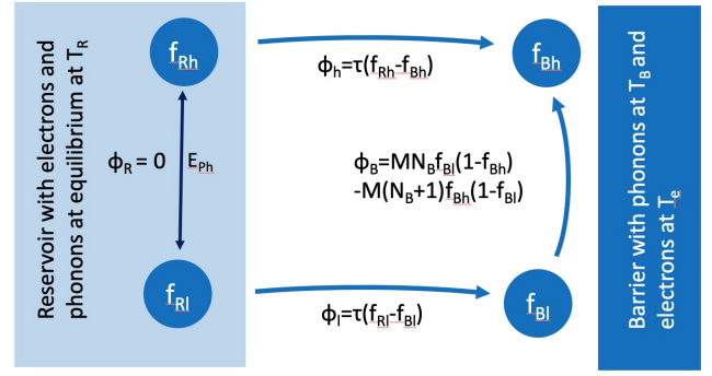
FIG. 13. (Color online) Schematic representation of an analytic model of the revolving effect based on electronic flux. Left rectangle represents the reservoir at equilibrium in which both electrons and phonons are at the same temperature, T_R . The right rectangle represents the barrier in which temperatures of electrons ( T_e ) and phonons ( T_B ) can be different. f_{Rl} and f_{Rh} are the Fermi-Dirac distributions in the reservoir of the low and high energy states, separated by the energy of a polar optical phonon ( E_{ph} ), respectively. Similarly, f_{Bl} and f_{Bh} are the electronic distributions at the barrier edge. In the reservoir and the barrier edge, the electronic fluxes between the low and high states, due to phonon absorption/emission are \phi_R and \phi_B respectively. M is the electron-phonon coupling, and N_B is the phonon's distribution at the barrier edge, given by the Bose-Einstein distribution. Finally, the fluxes between the reservoir and barrier states at high- and low-energy are \phi_h and \phi_l respectively. \tau is the transition rate between the reservoir and the barrier states (assumed constant at low and high energies).
