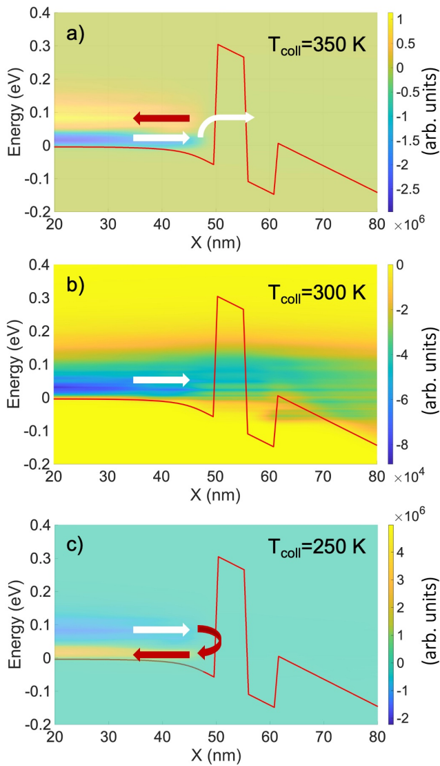
FIG. 11. (Color online) Electron current spectrum at V=0.1 V for the three collector temperatures shown in Fig.10: a) T_{\text{Coll}}=350 K, b) T_{\text{Coll}}=300 K, c) T_{\text{Coll}}=250 K. In the three cases, T_{\text{Emit}}=300 K. The solid red line represents the energy potential profile, while red and white arrows indicate the electron flow, reflection and transmission on the potential barrier.
