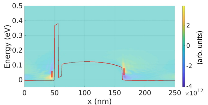
FIG. 3. (Color online) Derivative of the energy current spectrum (Eq. (11)). The yellow color regions represent the predominance of outgoing electrons, while blue color regions are those of incoming electrons. The up arrow indicates the promotion of low energy electrons to high energy electrons (i.e. phonon absorption). The down arrow indicates electron decay to lower energy (phonon emission).
