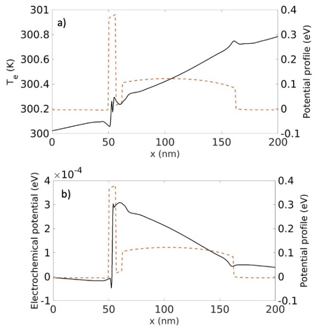
FIG. 5. (Color online) a) Non-equilibrium electron temperature along the device and b) corresponding electrochemical potential when applying lattice temperature gradient of 1K and no potential bias ( V=0 V).
