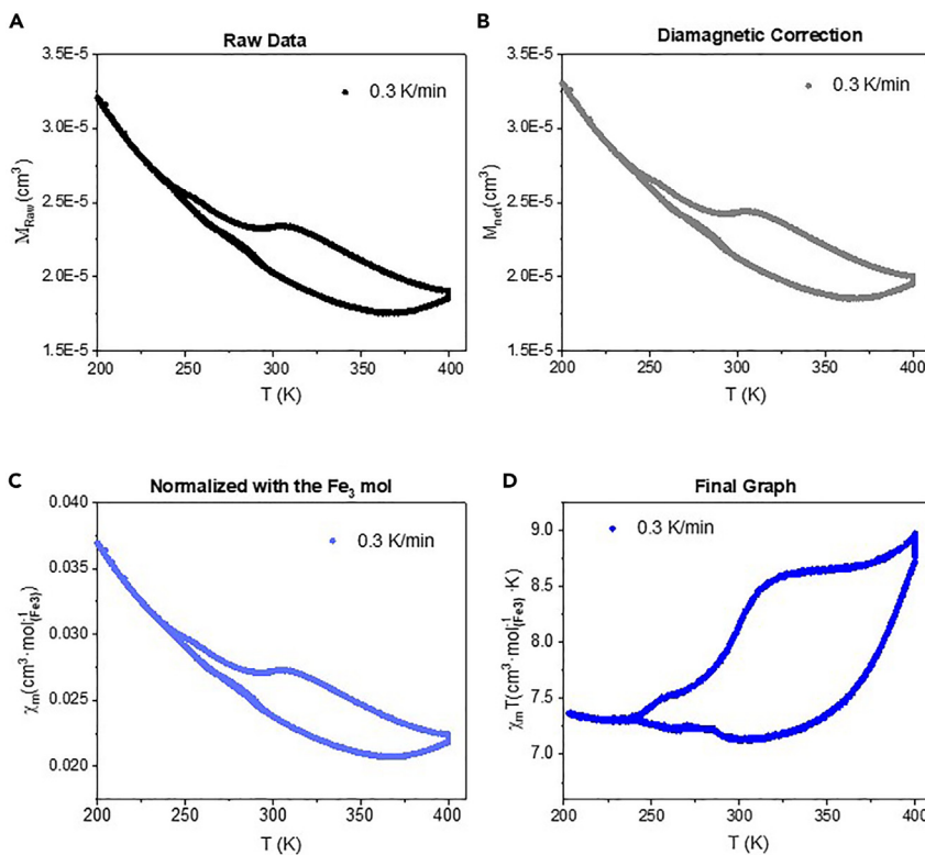
Figure 7. Data correction process for magnetic susceptibility cycle of Zn_{3(1-x)}Fe_{3(x)} ( x = 0.4 ) (A) Raw magnetization extracted from the SQUID measurements. (B) Net magnetization obtained after correction of the diamagnetic contribution of the sample holder. (C) Magnetization per mol of iron trimer. (D) Final graph representing magnetic susceptibility temperature product ( \chi_m \cdot T ) vs. temperature.
