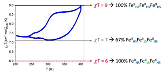
Figure 8. Magnetic susceptibility data in the 200–400 K range for Zn_{3(1-x)}Fe_{3(x)} , x = 0.4 (blue dots) The theoretical \chi_M T value for 100% of Fe_{HS}^{II}Fe_{LS}^{II}Fe_{HS}^{II} and Fe_{HS}^{II}Fe_{HS}^{II}Fe_{HS}^{II} is represented by red arrows.
