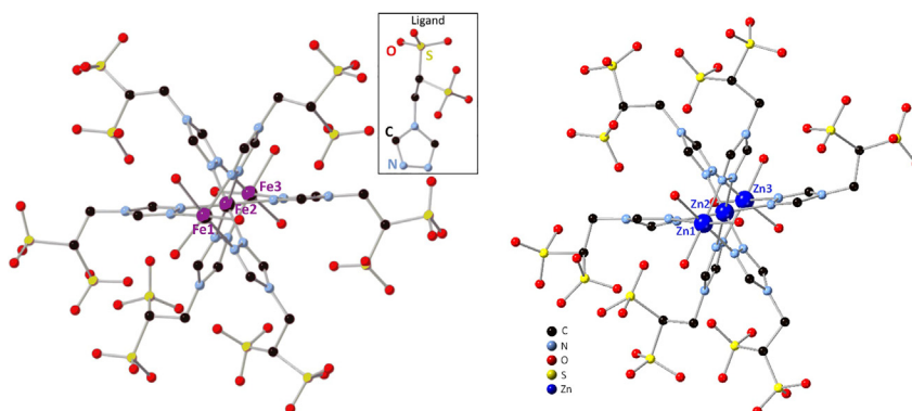
Figure 4. Representation of the molecular structure of Fe 3 (left) and Zn 3 (right)
