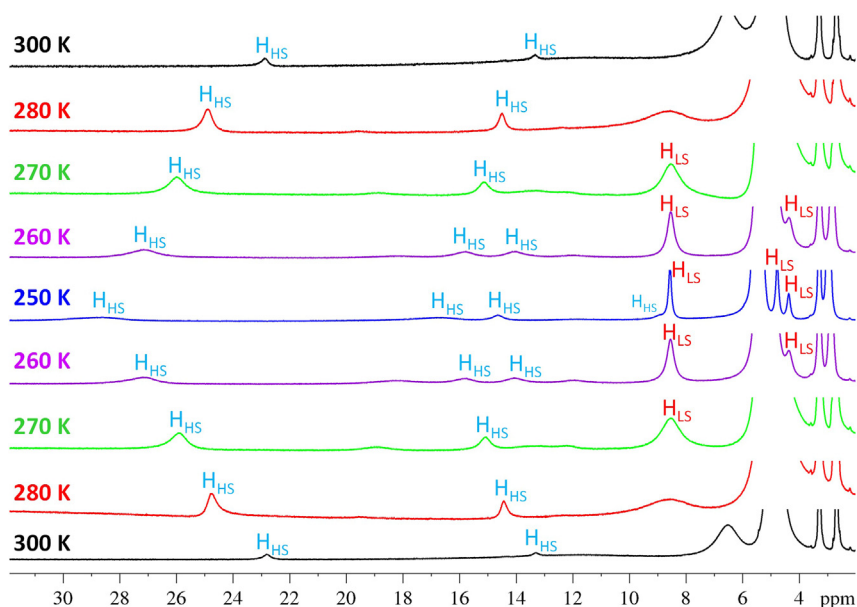
Figure 11. 1 H-NMR spectra of Fe 3 in D 2 O:CD 3 OD (3:4 v.v.) at 300–250 K temperature range The 1 H signals of the HS and LS species are defined as H HS and H LS , respectively.
