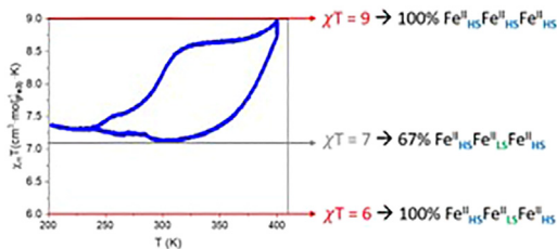
Figure 8. Magnetic susceptibility data in the 200–400 K range for Zn_{3(1-x)}Fe_{3(x)} , x = 0.4 (blue dots)
