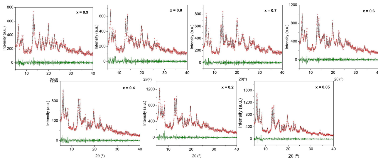
Figure 5. Pawley refinement (black line) of PXRD patterns (red circles) for Zn_3(1-x)Fe_3(x) The green line represents the difference between fitting and experimental data.
