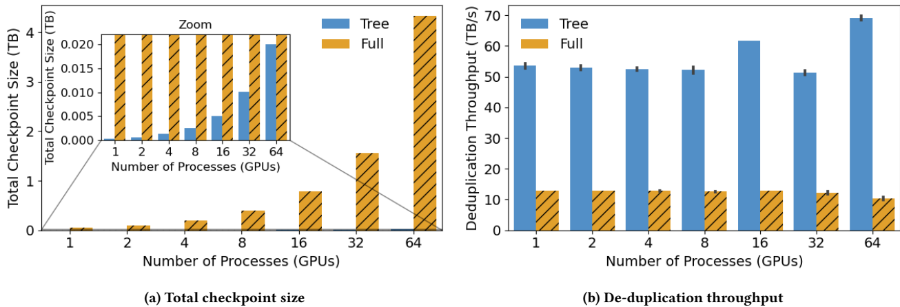
Figure 6: Strong scaling results with up to 64 GPUs using the Delaunay N24 input graph. Our method (Tree) achieves over two orders of magnitude reduction in checkpoint size compared with Full and retains a high throughput at scale.
