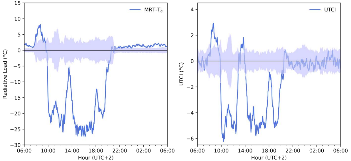
Figure 9: Average microclimatic effects of the site's conversion. ( MRT - T_a ): radiative load, ( UTCI ): UTCI -equivalent temperature.
