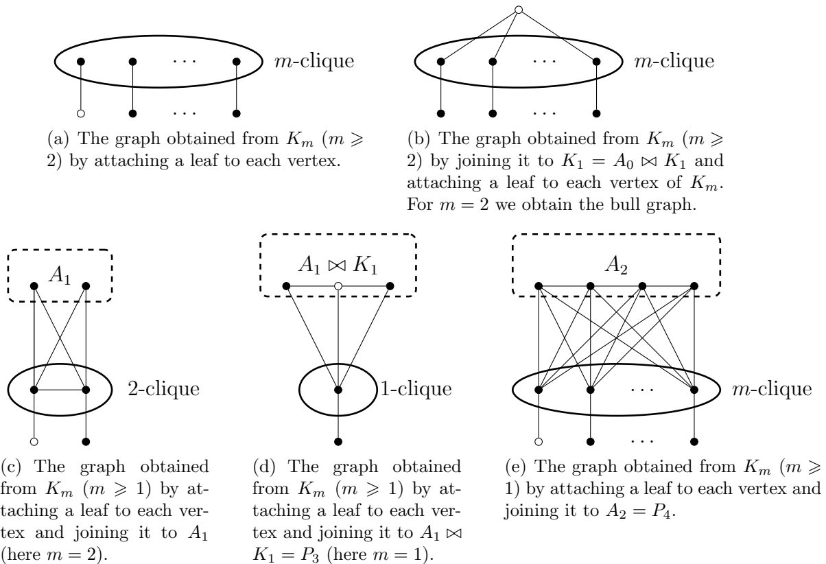
Figure 4: Some examples of graphs of order n with total dominating identifying code number n - 1 but a smaller identifying code. Black vertices form a minimum total dominating identifying code.
