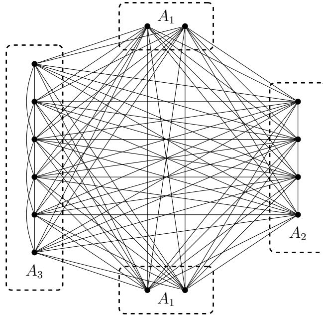
Figure 3: A graph in \mathcal{A}^* built from two copies of A_1 and from one copy of each of A_2 and A_3 .
