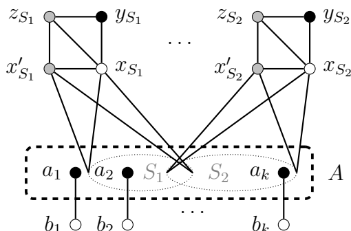
Figure 8: Sketch of the graph G_k built in Proposition 21, where S_1 and S_2 are two subsets of A of size at least 2. The black vertices form an optimal locating-dominating set, while the black and gray vertices together form an optimal total dominating identifying code.
