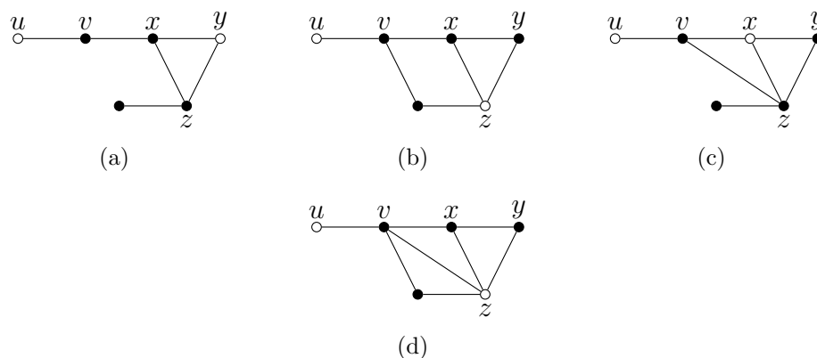
Figure 5: The possibilities for graph G when G'' is isomorphic to P_3 , in part (3) of the proof of Lemma 8. The black vertices form total dominating sets of size n - 2 .
