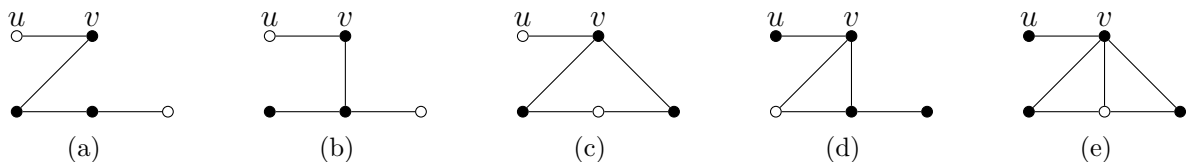
Figure 6: The possibilities for graph G when G - u - v is isomorphic to P_3 , in the proof of Theorem 5. The black vertices form total dominating identifying codes.
