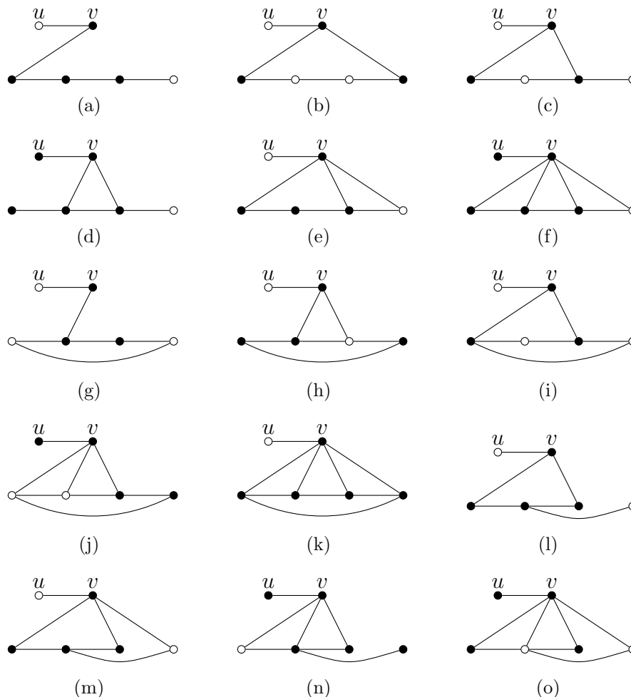
Figure 7: The possibilities for graph G when G - u - v is isomorphic to P_4 , C_4 or K_{1,3} , in the proof of Theorem 5. The black vertices form total dominating identifying codes.
