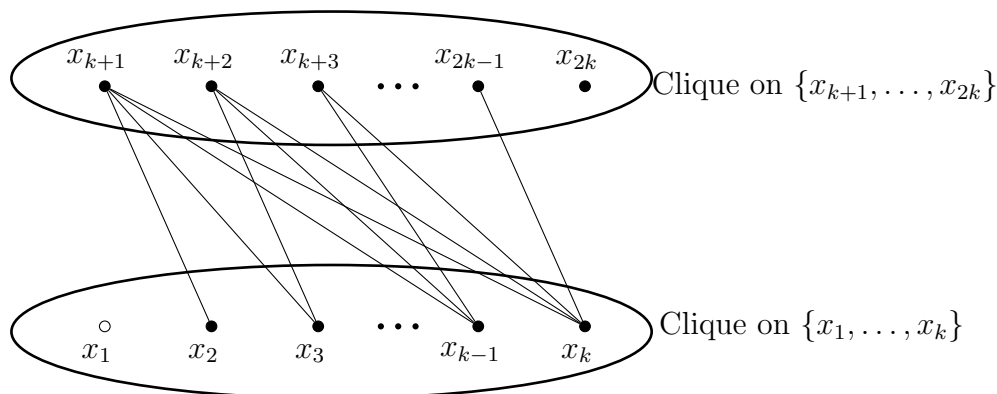
Figure 2: The graph A_k of order n = 2k has total dominating identifying code number n - 1 (the black vertices form an optimal total dominating identifying code).
