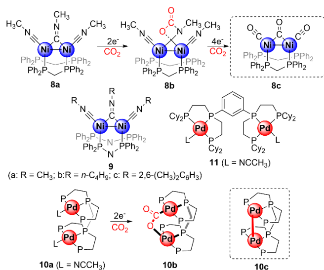
Figure 1. Phosphine ligand based homobimetallic catalysts.
