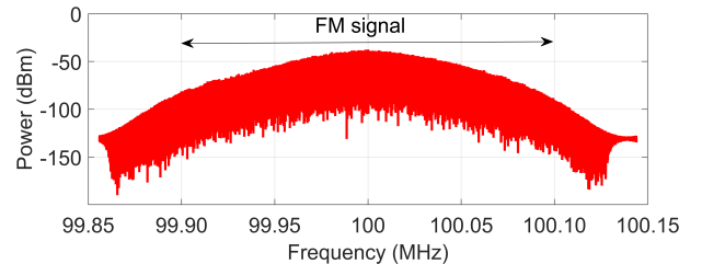
Fig. 3. Frequency spectrum of the RF signal obtained in Keysight's ADS by performing FM modulation of a 100 MHz carrier.
