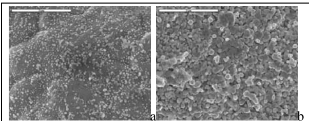
Fig. 5. SEM visualization (a) 2 wt % Ni coating (b) 10 wt % Ni coating on Al particle.
