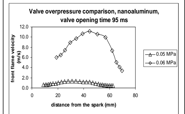
Fig. 7b. Flame front velocity of nanoAl particles cloud for different valve overpressure.
