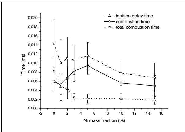
Fig. 4. Ignition delay, combustion and total combustion times of Ni-coated Al particles in air as a function of Ni mass fraction.
