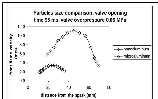
Fig. 7c. Flame front velocity of nanoAl and microAl particles cloud
