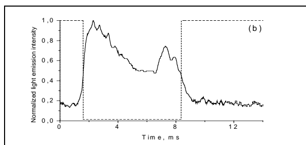
Fig. 3b. Light mission during ignition and combustion of Al/Ni (14.4 wt.% Ni) particles in air. The dashed line shows the laser monitoring sequence
