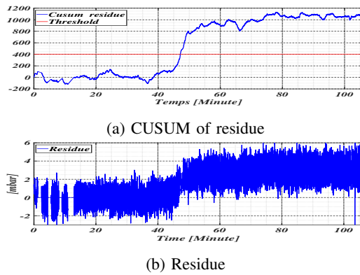
Fig. 10: Flooding detection
