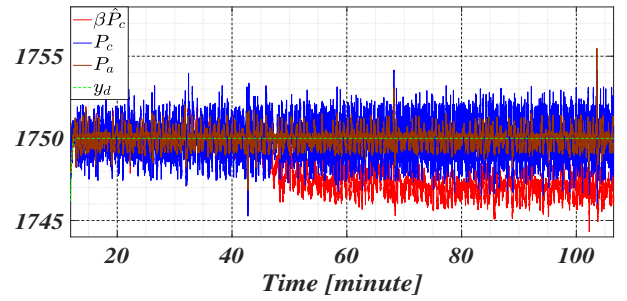
Fig. 9: Measured and estimated cathode inlet pressure
