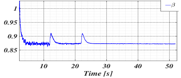
Fig. 2: Evolution of \beta in fault free case
