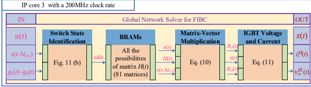
Fig. 12. Hardware implementation of the global network solver for FIBC.
